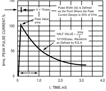
FIG. 3 - PULSE WAVEFORM
